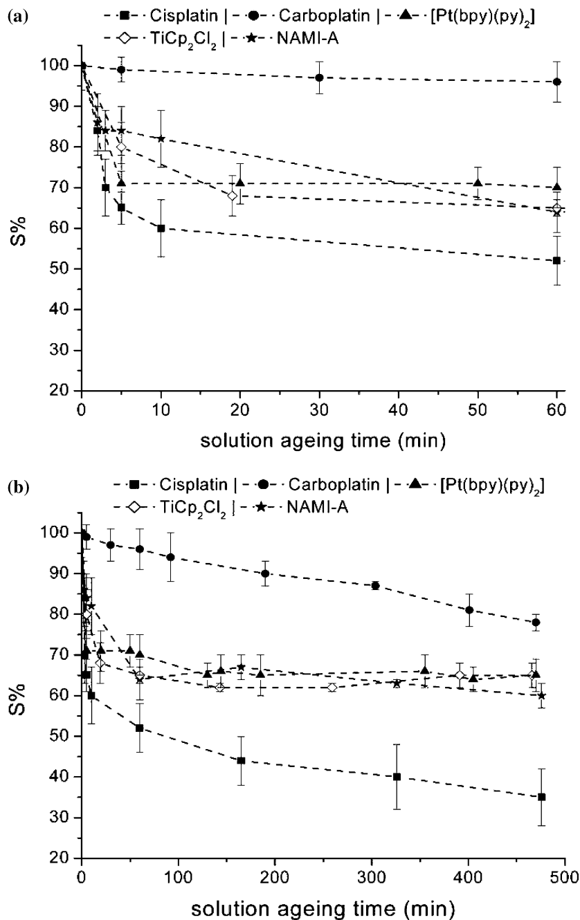
Figure 3. Guanine oxidation signal S% vs. solution ageing time for 0.5 mM solution of the metal complexes in 0.25 M phosphate buffer (pH = 7.4) and 5 mM NaCl: (a) 0–60 min time range, (b) 0–500 min time range.
